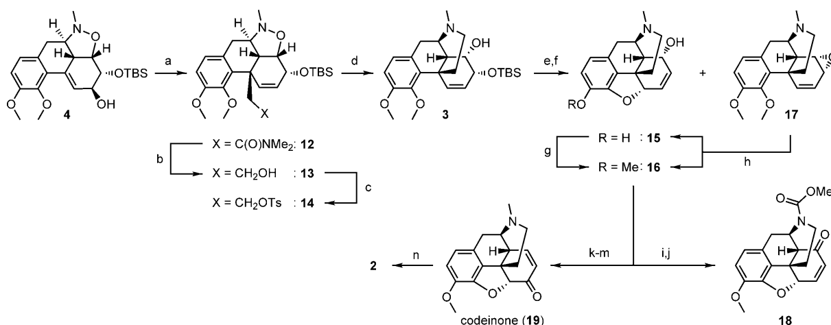
Scheme 3. Completion of both formal and total syntheses of (±)-codeine. a) \text{MeC}(\text{OMe})_2\text{NMe}_2 , toluene, Dean–Stark trap, reflux, 87%; b) LDA, \text{BH}_3\cdot\text{NH}_3 , 0^\circ\text{C} \rightarrow \text{RT} , 97%; c) p\text{TsCl} , \text{Et}_3\text{N} , cat. DMAP, \text{CH}_2\text{Cl}_2 , 0^\circ\text{C} \rightarrow \text{RT} ; d) \text{EtOH}/\text{EtOAc} (3:1), \text{Et}_3\text{N} , Raney Ni, 1 atm \text{H}_2 , RT, 86% (2 steps); e) TBAF, THF, 0^\circ\text{C} , 100% crude; f) 1. \text{BBr}_3 , \text{CH}_2\text{Cl}_2 , -65^\circ\text{C} , 2. aq. \text{NaHCO}_3 , RT, 15% 16 + 19% 15 + 16% 17 (2 steps); g) \text{Me}_3\text{NPhCl} , NaOEt, toluene, reflux, 80%; h) 1. \text{BBr}_3 , \text{CH}_2\text{Cl}_2 , -65^\circ\text{C} , 2. aq. \text{NaHCO}_3 , RT, 37% 16 + 16% 15 ; i) DMP, \text{NaHCO}_3 , \text{CH}_2\text{Cl}_2 , RT, 91%; j) \text{ClC}(\text{O})\text{OMe} , \text{NaHCO}_3 , \text{CHCl}_3 , reflux, 93%; k) \text{SOCl}_2 , 0^\circ\text{C} \rightarrow \text{RT} , 77% crude; l) 1,4-dioxane/water (1:1), 100^\circ\text{C} , microwave irradiation, 72%; m) DMP, \text{NaHCO}_3 , \text{CH}_2\text{Cl}_2 , RT, 29% 19 + 30% pseudocodeine; n) \text{NaBH}_4 , MeOH, RT, 99%. DMP = Dess–Martin periodinane, LDA = lithium diisopropylamide, TBAF = tetrabutylammonium fluoride.
