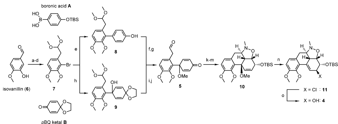
Scheme 2. Facile preparation of the highly functionalized phenanthrene 4 . a) \text{Br}_2 , cat. Fe powder, NaOAc, HOAc, RT, 92%; b) aq. KOH, \text{Me}_2\text{SO}_4 , 50^\circ\text{C} , 95%; c) \text{Ph}_3\text{PCH}_2\text{OMeCl} , \text{KO}^t\text{Bu} , THF, 0^\circ\text{C} ; d) cat. p\text{TsOH}\cdot\text{H}_2\text{O} , MeOH, \text{HC}(\text{OMe})_3 , reflux, 95% (2 steps); e) 1. boronic acid A , \text{K}_2\text{CO}_3 , 1,4-dioxane/water (7:3), cat. BHT, 2.6 mol% [\text{Pd}_2(\text{dba})_3] , 5.2 mol% \text{PCy}_3 , 80^\circ\text{C} , 2. aq. NaOH, 50^\circ\text{C} , 95% (2 steps); f) PIDA, MeOH, \text{HC}(\text{OMe})_3 , RT, 66% + 24% o -quinone dimethylacetal; g) cat. CAN, MeCN/borate buffer (1:1), pH 5–6, 60^\circ\text{C} , 97% crude; h) 1. BuLi, THF, -78^\circ\text{C} , 2. pBQ ketal B , -78^\circ\text{C} \rightarrow -70^\circ\text{C} , 70%; i) NaH, MeI, THF, 30^\circ\text{C} ; j) cat. CAN, MeCN/borate buffer (1:1), pH 5–6, 60^\circ\text{C} , 104% crude; k) \text{MeNHOH}\cdot\text{HCl} , \text{NaHCO}_3 , \text{MgSO}_4 , MeCN, 0^\circ\text{C} ; l) 1. L-selectride, THF, -78^\circ\text{C} , 2. MeOH, -78^\circ\text{C} \rightarrow \text{RT} , 3. aq. NaOH, \text{H}_2\text{O}_2 , RT; m) TBSCl, imidazole, cat. DMAP, \text{CH}_2\text{Cl}_2 , RT, 80% (3 steps); n) 1. \text{BCl}_3 , \text{CH}_2\text{Cl}_2 , -78^\circ\text{C} , 2. \text{Et}_3\text{N} , MeOH, -78^\circ\text{C} \rightarrow \text{RT} ; o) ZnO, acetone/water (4:1), 80^\circ\text{C} , 76% (2 steps). BHT = 2,6-di- tert -butyl-4-methylphenol, CAN = ceric ammonium nitrate, Cy = cyclohexyl, dba = dibenzylideneacetone, DMAP = 4-( N,N -dimethylamino)pyridine, L-selectride = lithium tri- sec -butylborohydride, TBS = tert -butyldimethylsilyl, pTs = p -toluenesulfonyl.
