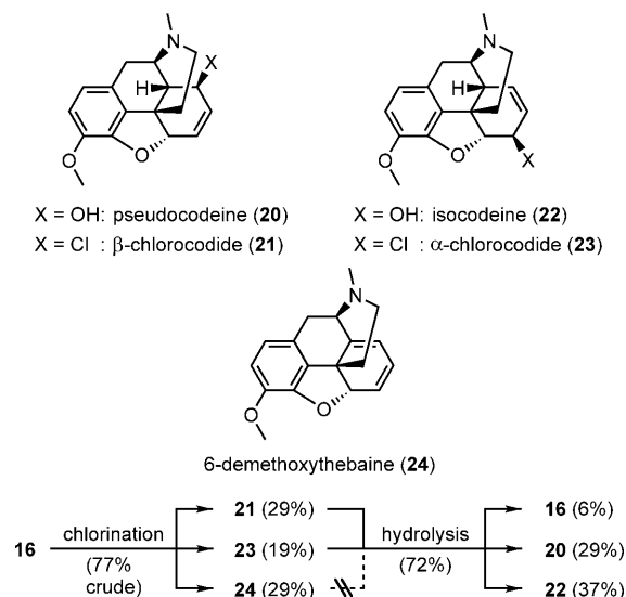
Scheme 4. A closer look at the allylic transposition.
