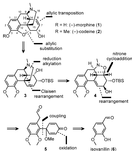
Scheme 1. Pentacyclic morphine ( 1 ) and retrosynthetic analysis of the applied phenanthrene route.
